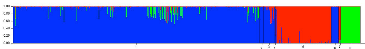
Figure 4. STRUCTURE bar graph of seven C. mindorensis populations and one C. porosus population at K -max, K = 3 clusters.
