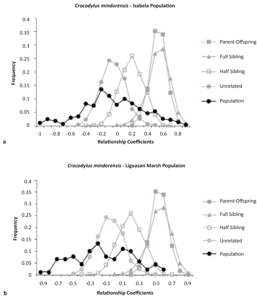
Figure 1. Relationship coefficient distributions of the two extant Crocodylus mindorensis populations from a - Isabela and b - Liguasan Marsh overlayed on a simulation of 10,000 individuals of known relationships by pedigree verification (Queller & Goodnight 1989).
