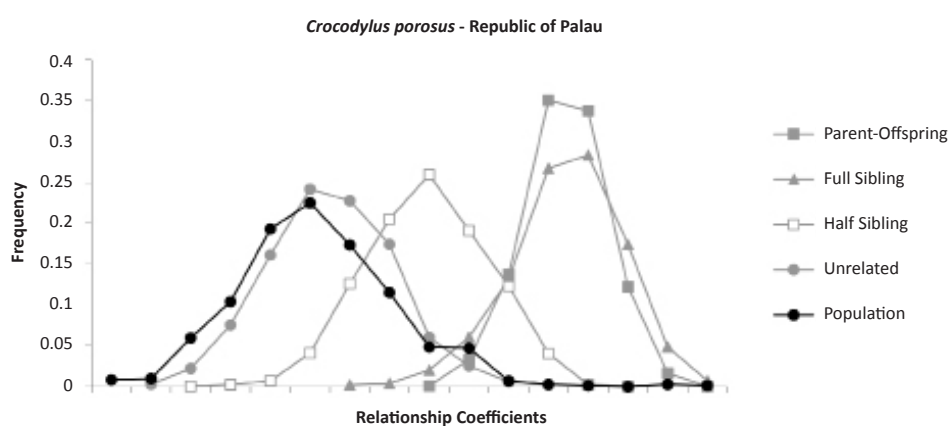
Figure 2. Relationship coefficient distributions of the Crocodylus porosus population from the Republic of Palau overlayed on a simulation of 10,000 individuals of known relationships by pedigree verification (Queller & Goodnight 1989).
