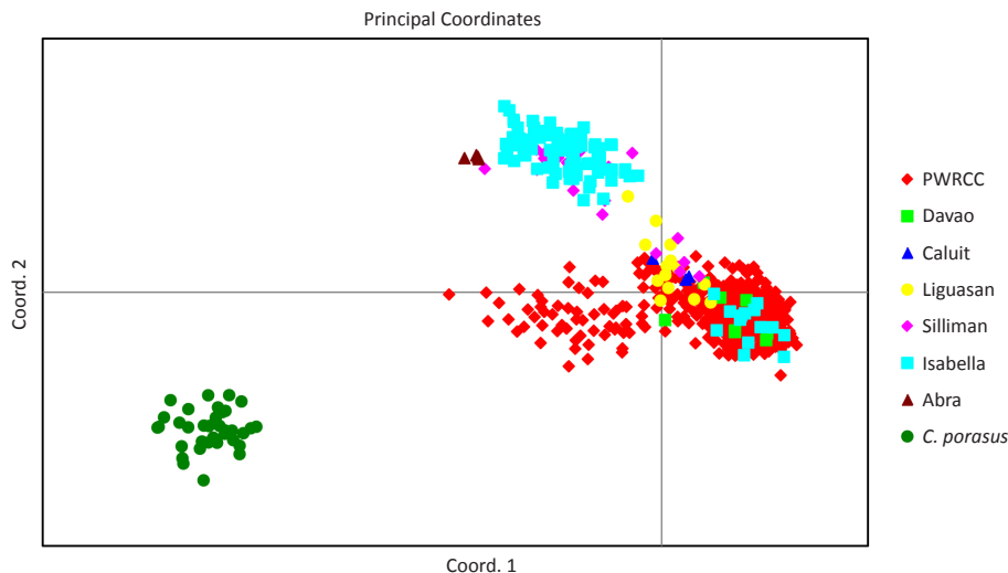
Figure 5. Principal Coordinate Analysis (PCoA) of the Crocodylus mindorensis populations sampled in the Philippines and the C. porosus population in Republic of Palau indicating the southern populations, the group of PWRCC C. mindorensis individuals with C. porosus introgression (red diamond cluster towards the C. porosus cluster) and the northern populations including individuals sampled in Isabela that were introduced from PWRCC (blue squares over the red diamond background).
