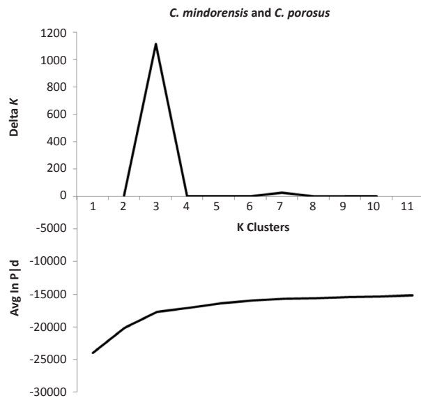
Figure 3. Evanno et al.'s (2005) \Delta K and chart of the average logarithm of the probability of the data for K -max, K = 3 , for seven populations of C. mindorensis and one population of C. porosus .
